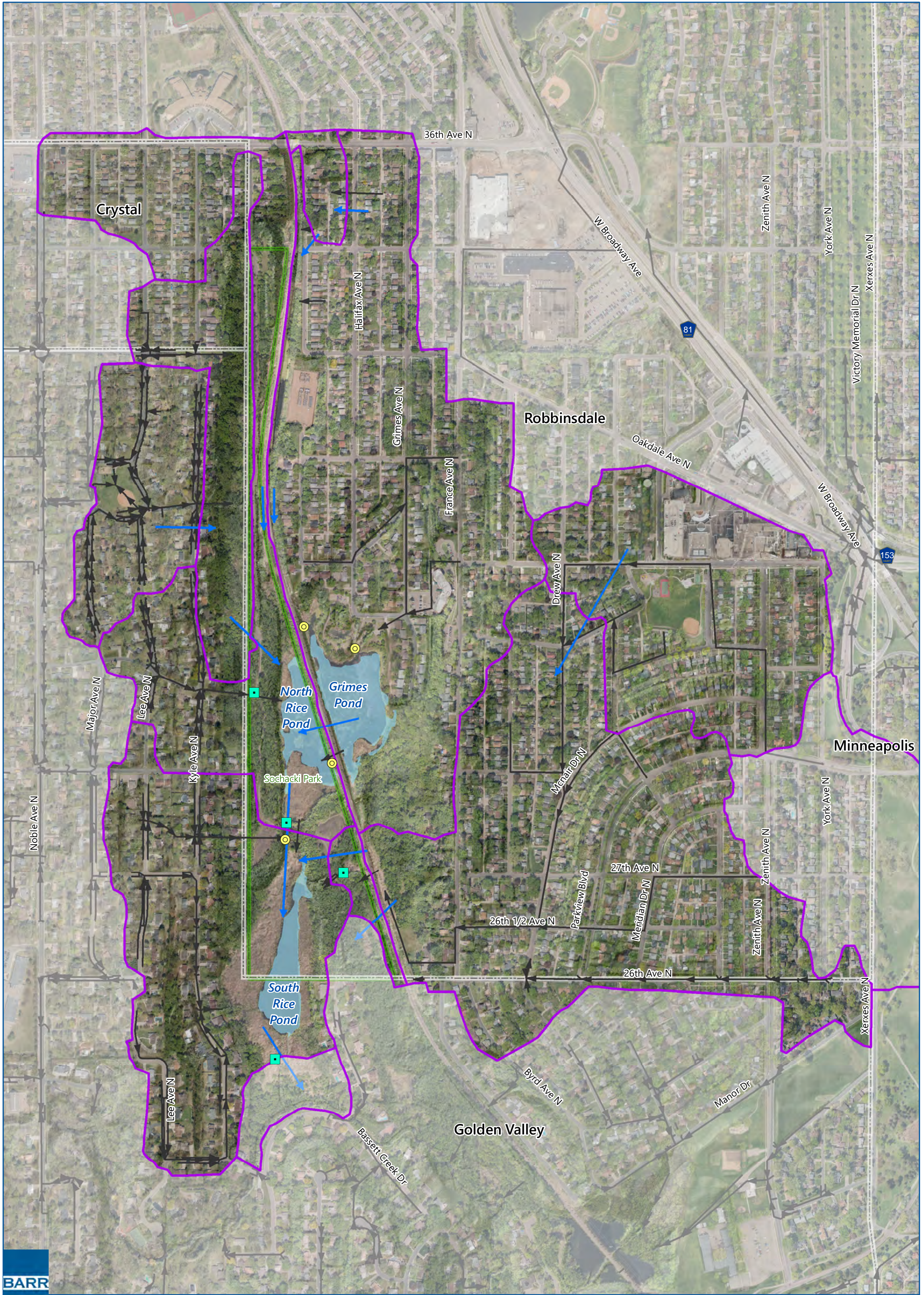
SUBWATERSHEDS & STORM SEWER Sochacki Park Subwatershed Assessment Three Rivers Park District FIGURE 1
